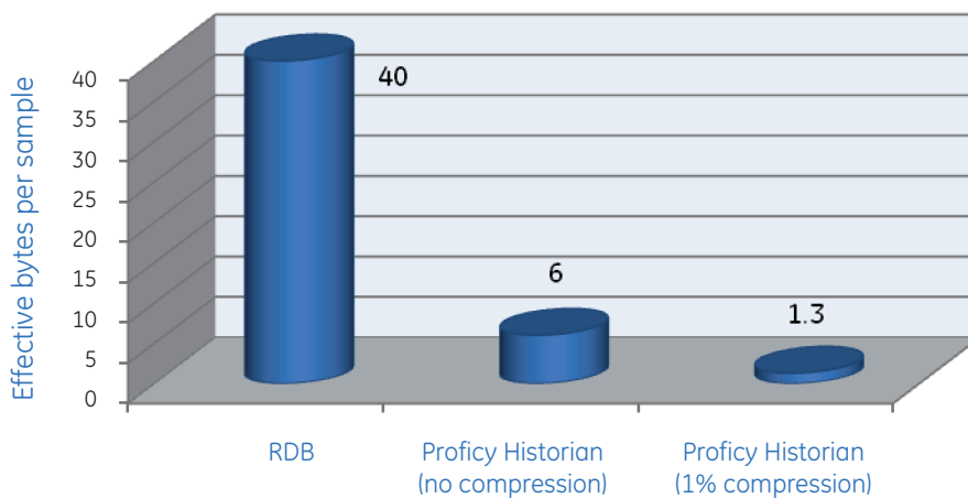
Comparing the disk space efficiency of an RDB vs. Proficy Historian†
